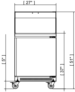
APTM-72-30 FRONT
