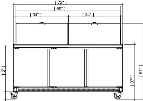
APTM-72-30 FRONT
