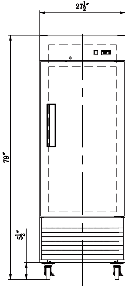
Front View
