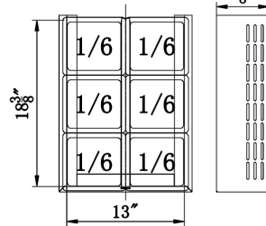
Lower drawer(right)
