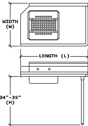
Right Side
